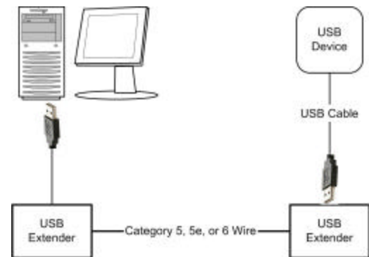
Typical USB Extender Installation
